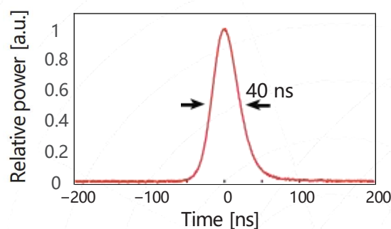
Typical pulse shape
